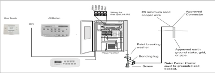
Figure 8. Wiring Configuration
