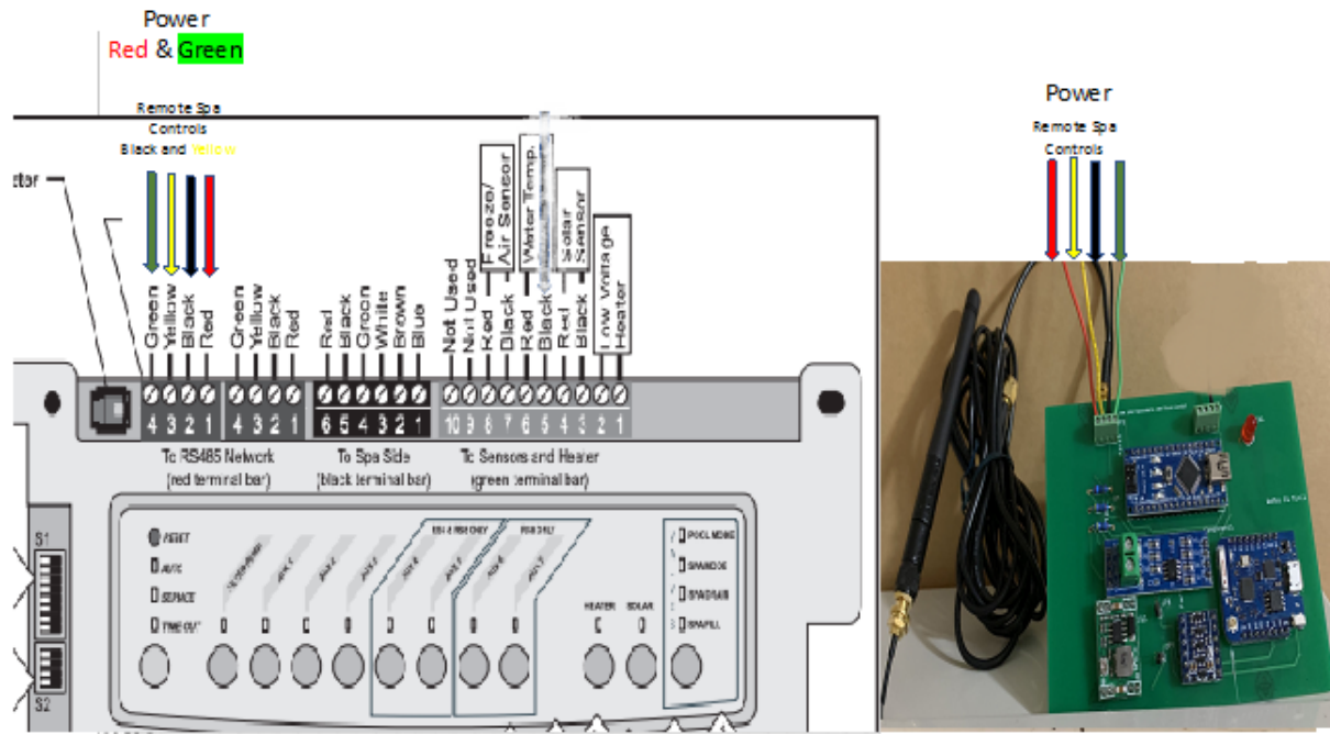
Wiring Diagram Figure Below
